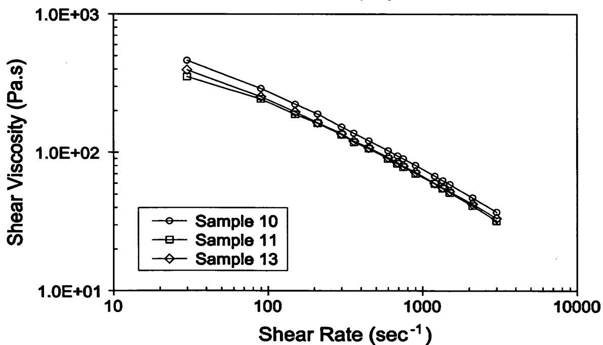
Fig. 12 Shear Viscosity of Plasticized Propylene Random Copolymers
